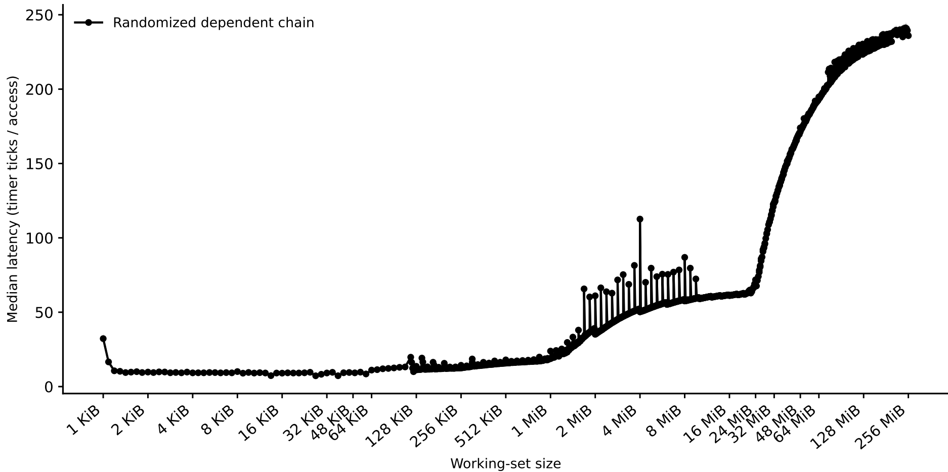
hazel_icelake_6326/capacity_rerun: capacity sweep (dependent pointer chase) (Phase I timing-only, auto pipeline)
