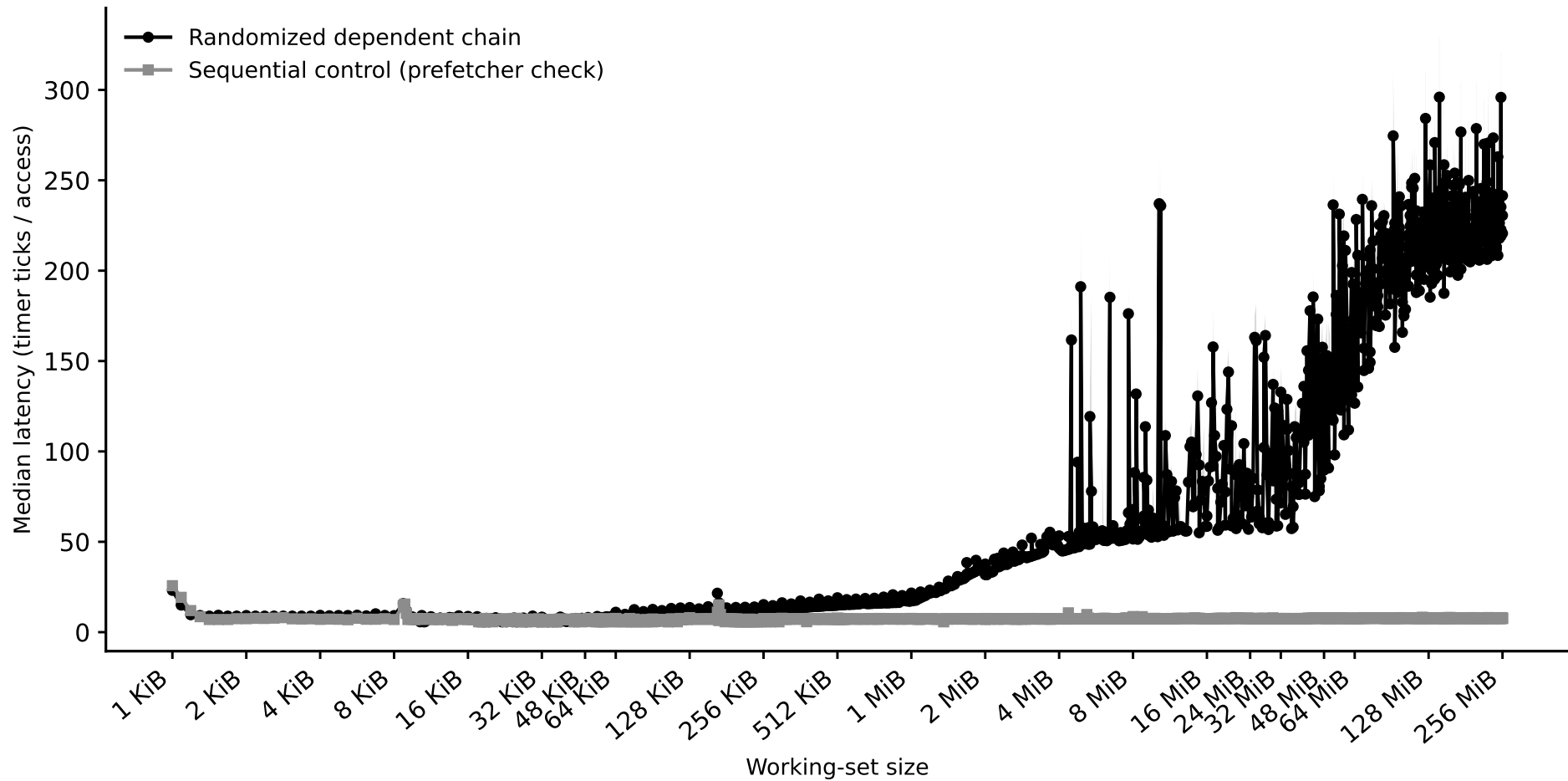
hazel_icelake_8358/capacity_rerun2: capacity sweep (dependent pointer chase) (Phase I timing-only, auto pipeline)
