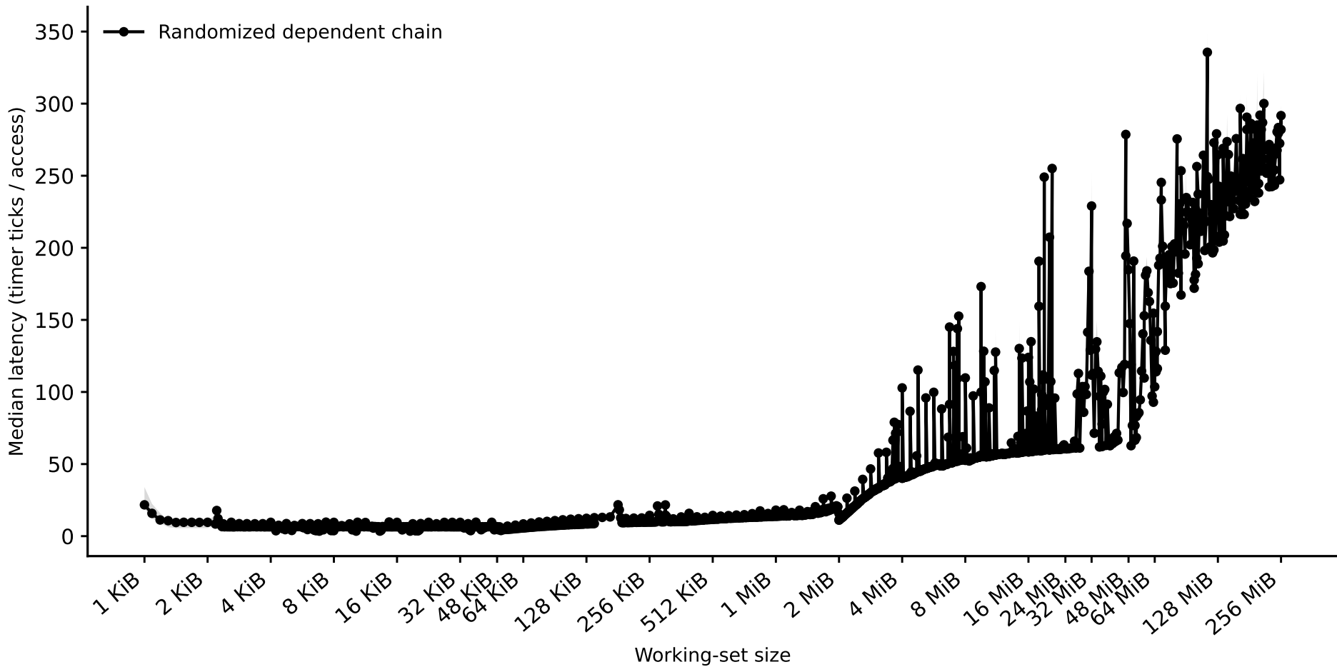
hazel_sapphirerapids: capacity sweep (dependent pointer chase) (Phase I timing-only, auto pipeline)
