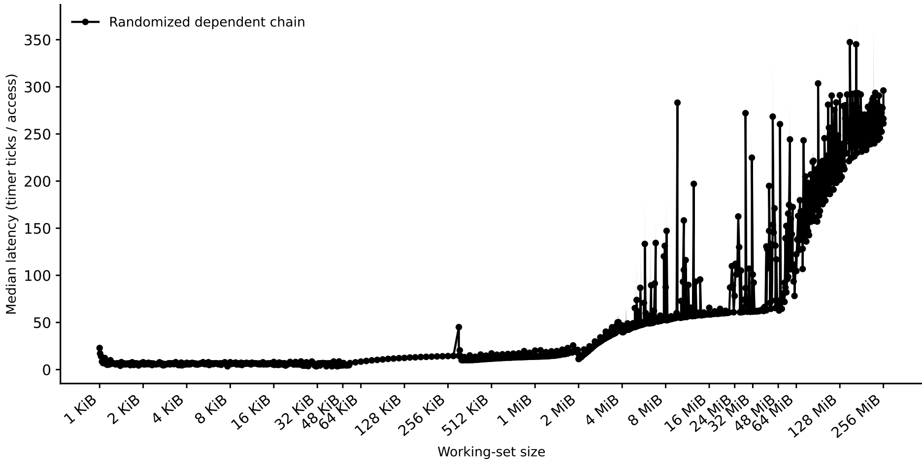
hazel_sapphirerapids/capacity_rerun: capacity sweep (dependent pointer chase) (Phase I timing-only, auto pipeline)
