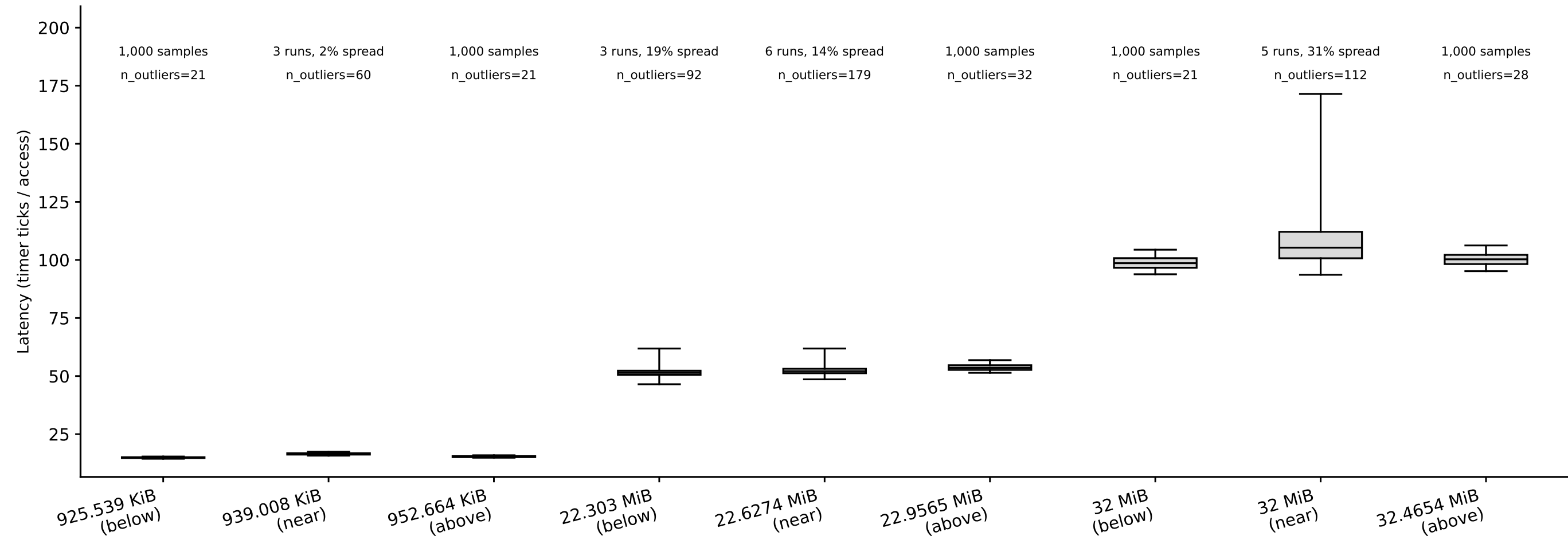
hazel_skylake/capacity_rerun: capacity box plots, random pattern (whiskers = p5/p95) (Phase I timing-only, auto pipeline) tested boundaries: 939.008 KiB, 22.6274 MiB, 32 MiB
