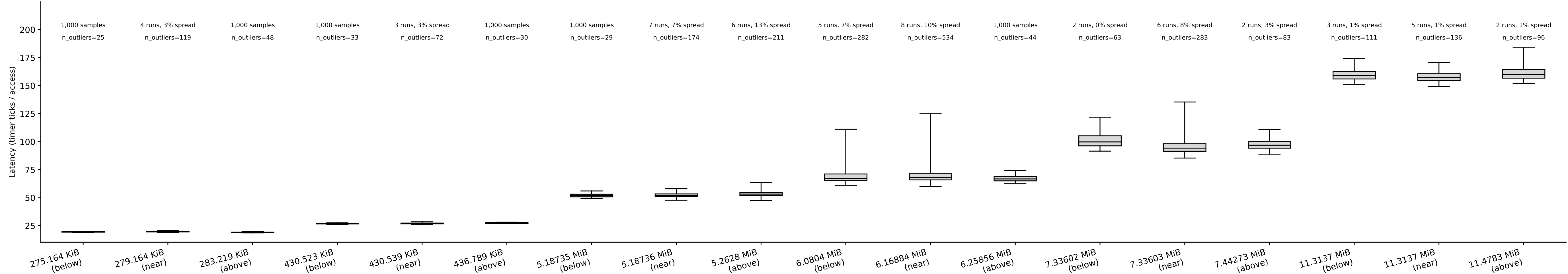
ookay: capacity box plots, random pattern (whiskers = p5/p95) tested boundaries: 279.164 KiB, 430.539 KiB, 5.18736 MiB, 6.16884 MiB, 7.33603 MiB, 11.3137 MiB
