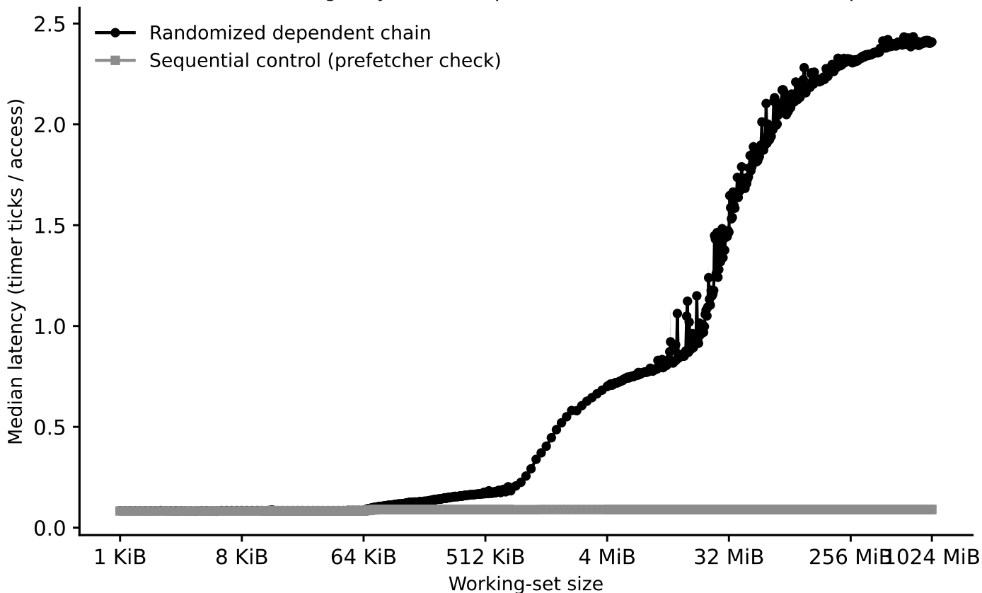
thunderbird: capacity sweep (dependent pointer chase) (Phase I timing-only, full sweep incl. manual dense+tail follow-up)
