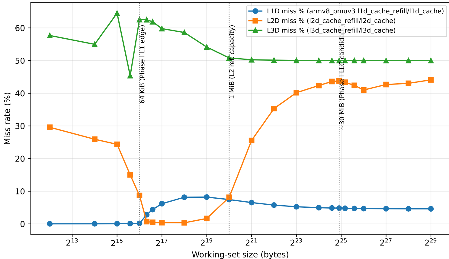
Thunderbird — PMU miss-rate sweep vs. working-set size (Phase II)
