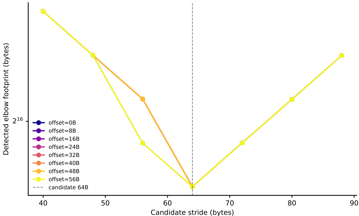
artemisia: line-size elbow vs. stride, by node-0 offset (Phase I timing-only, level boundary=49152B, step-4 alignment refinement)
