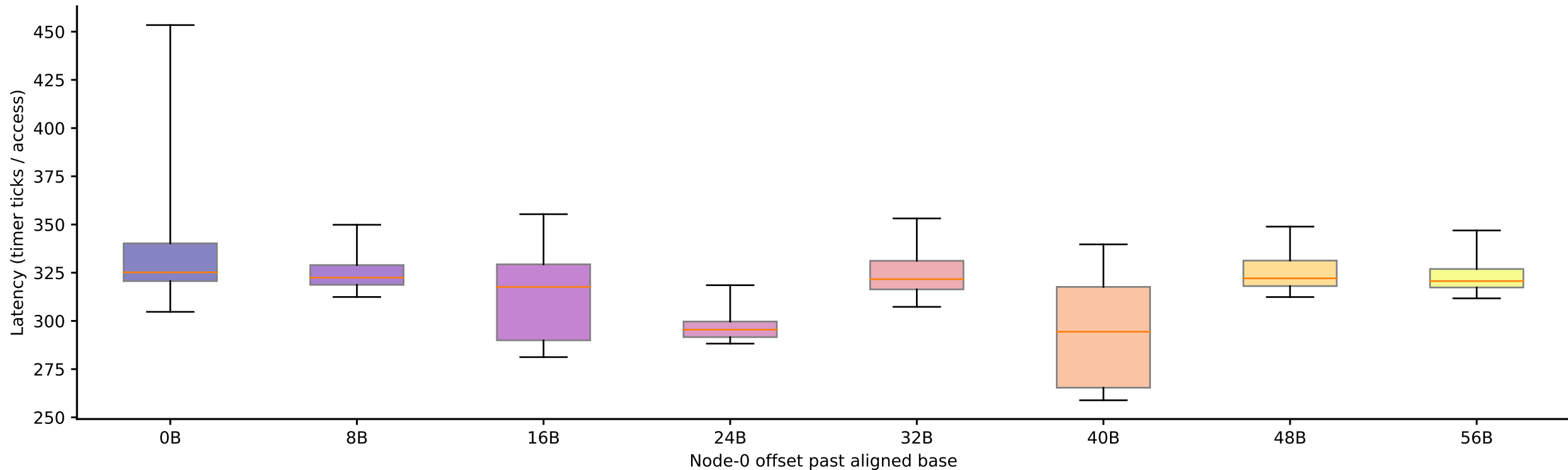
charnwood: candidate stride 64 B at footprint 20.1587 MiB, by offset (Phase I timing-only, level boundary=8388608B, step-4 alignment refinement)
