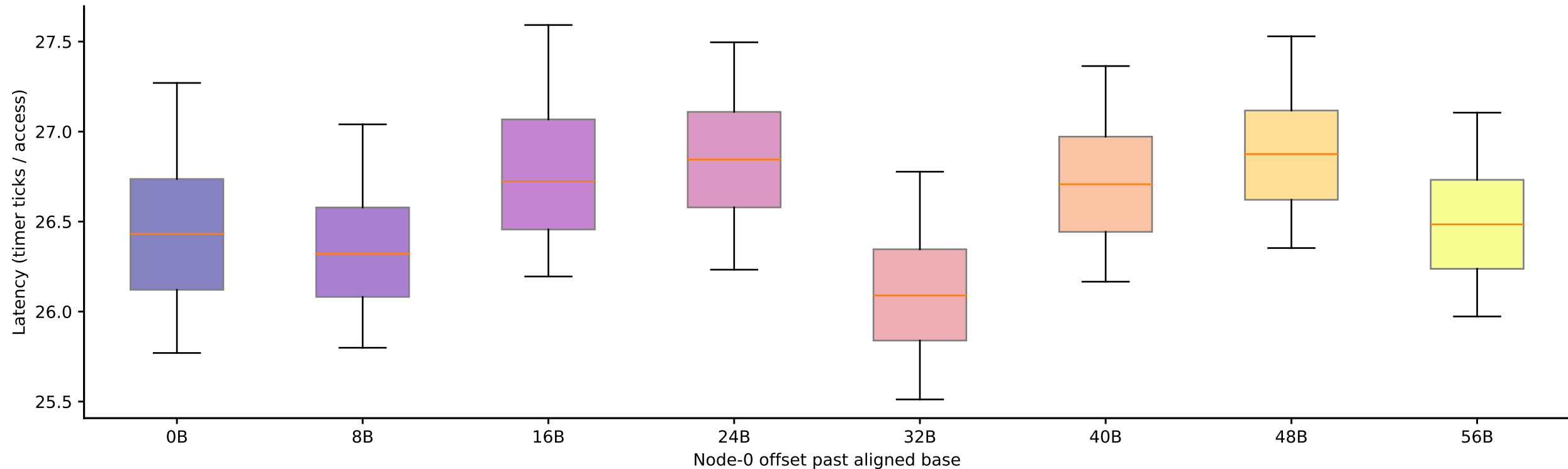
crux: candidate stride 64 B at footprint 512 KiB, by offset (Phase I timing-only, level boundary=262144B, step-4 alignment refinement)
