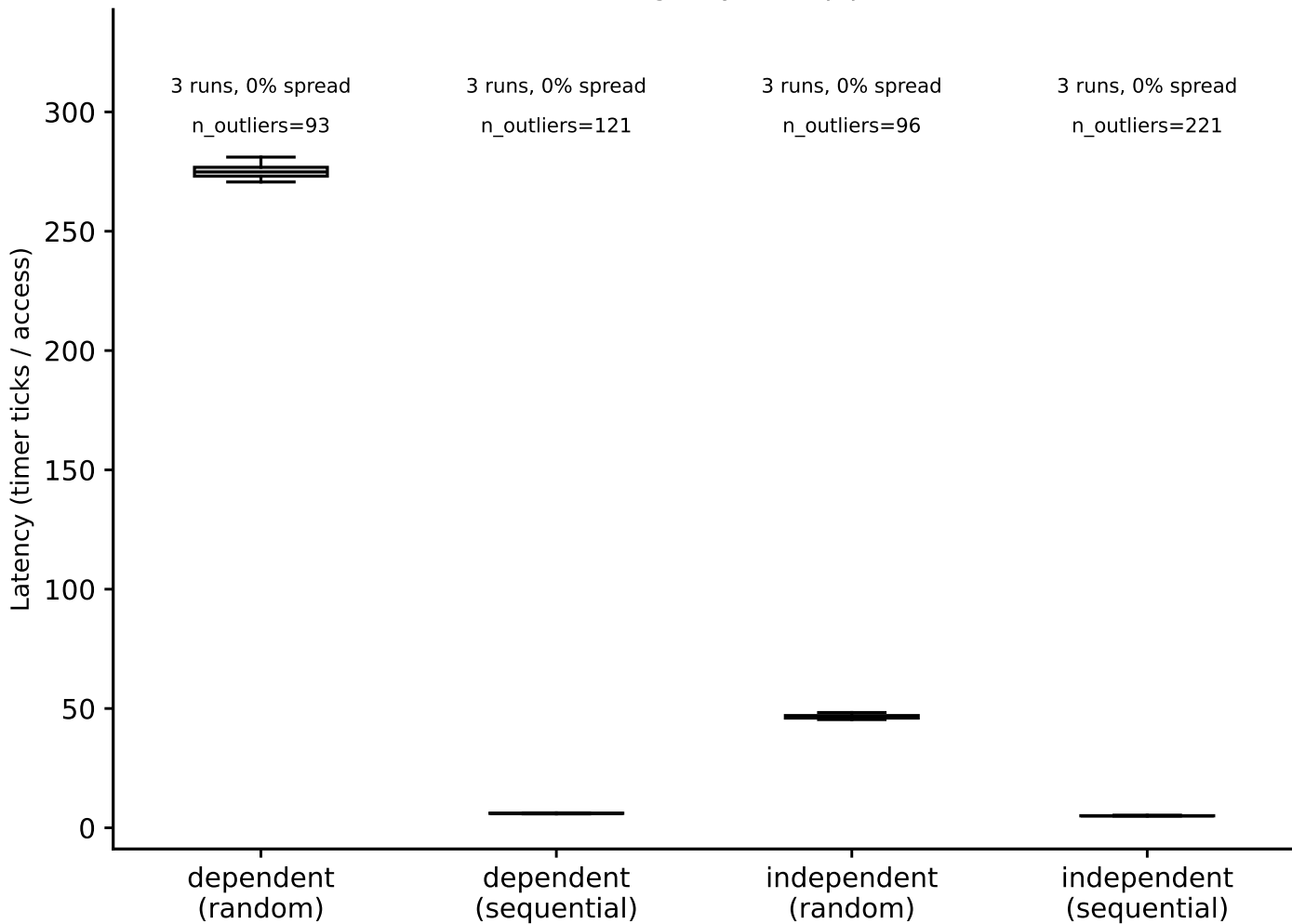
skylark: hit-latency box plots, DRAM (footprint=512 MiB) (Phase I timing-only, auto pipeline)
