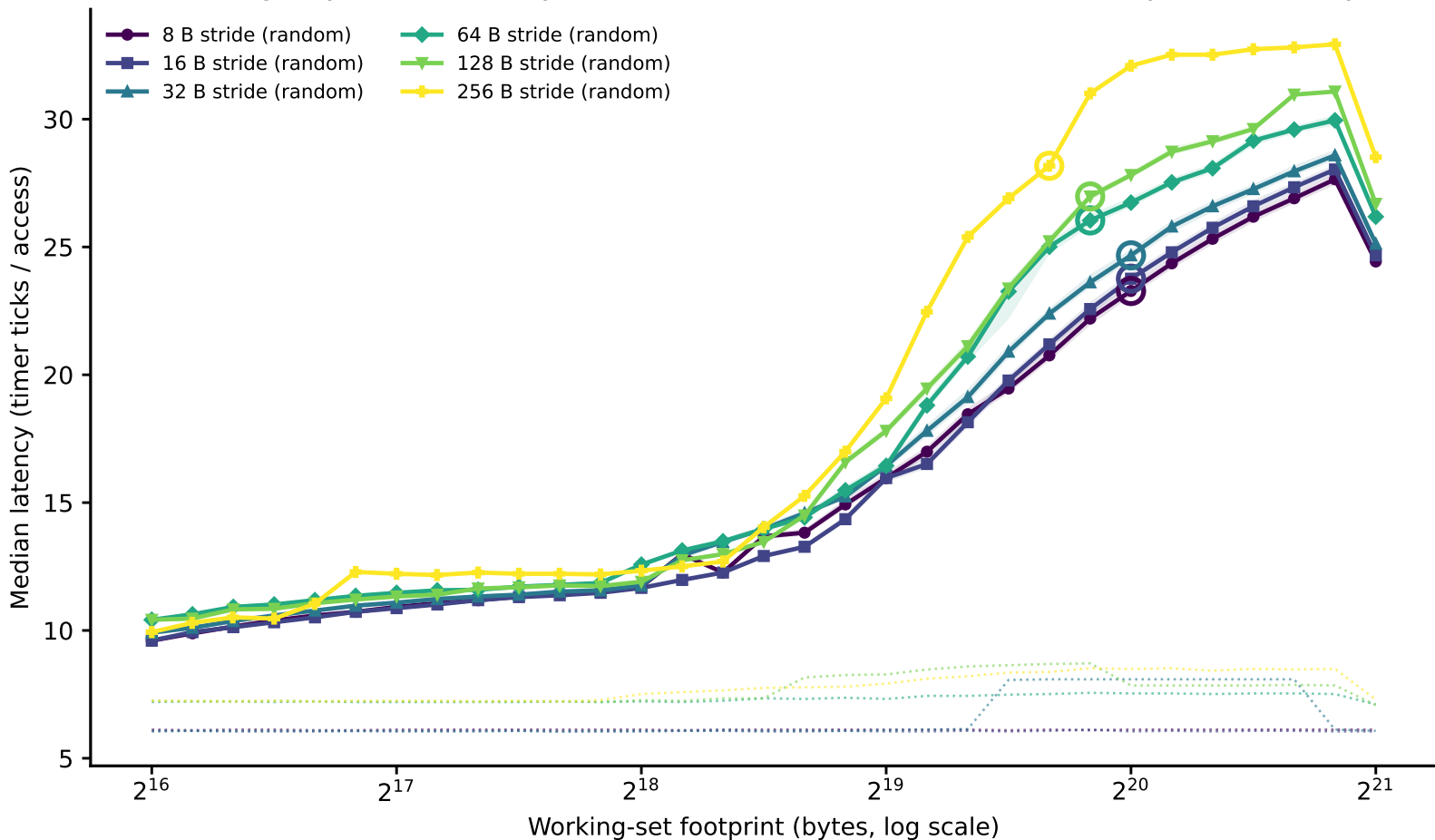
skylark: line-size family of curves (dependent pointer chase) (Phase I timing-only, level boundary=524288B window=[65536,2097152], family-of-curves-only rerun)
