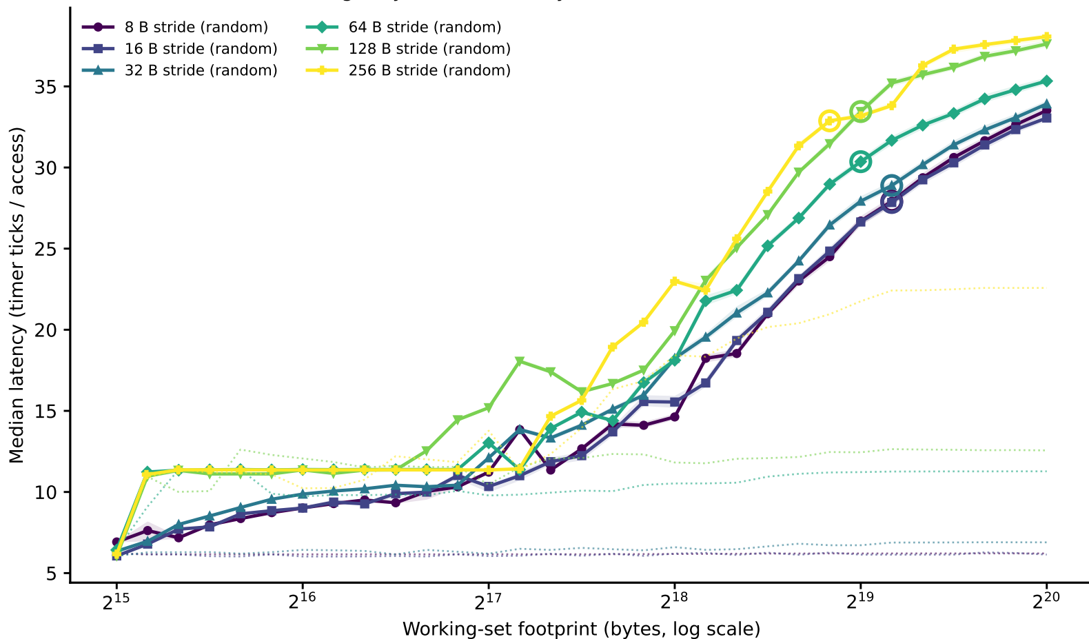
upgrade: line-size family of curves (dependent pointer chase) (Phase I timing-only, level boundary=262144B window=[32768,1048576])
