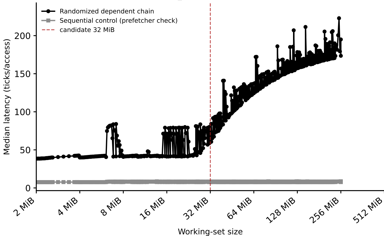
hazel_broadwell: LLC zoom
