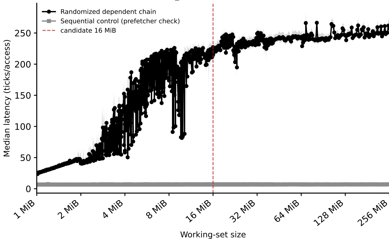
hazel_cascadelake: LLC zoom
