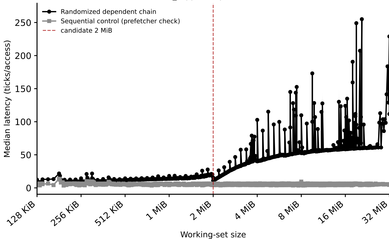
hazel_sapphirerapids: L2 zoom
