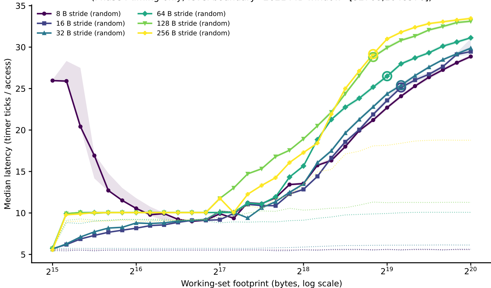
crux: line-size family of curves (dependent pointer chase) (Phase I timing-only, level boundary=262144B window=[32768,1048576])
