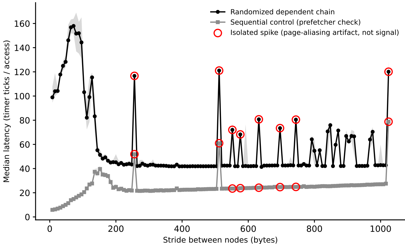
crux: line-size sweep (dependent pointer chase), footprint=16 MiB (Phase I timing-only, level boundary=8388608B, single-curve method)
