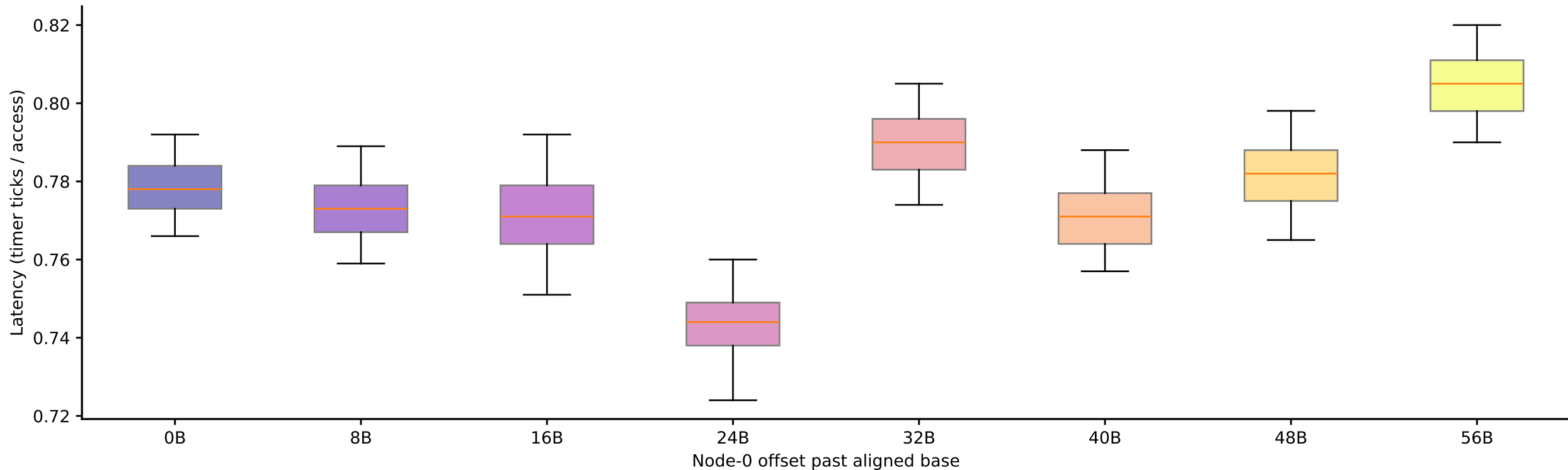
thunderbird: candidate stride 64 B at footprint 1.58734 MiB, by offset (Phase I timing-only, level boundary=1048576B, step-4 alignment refinement)
