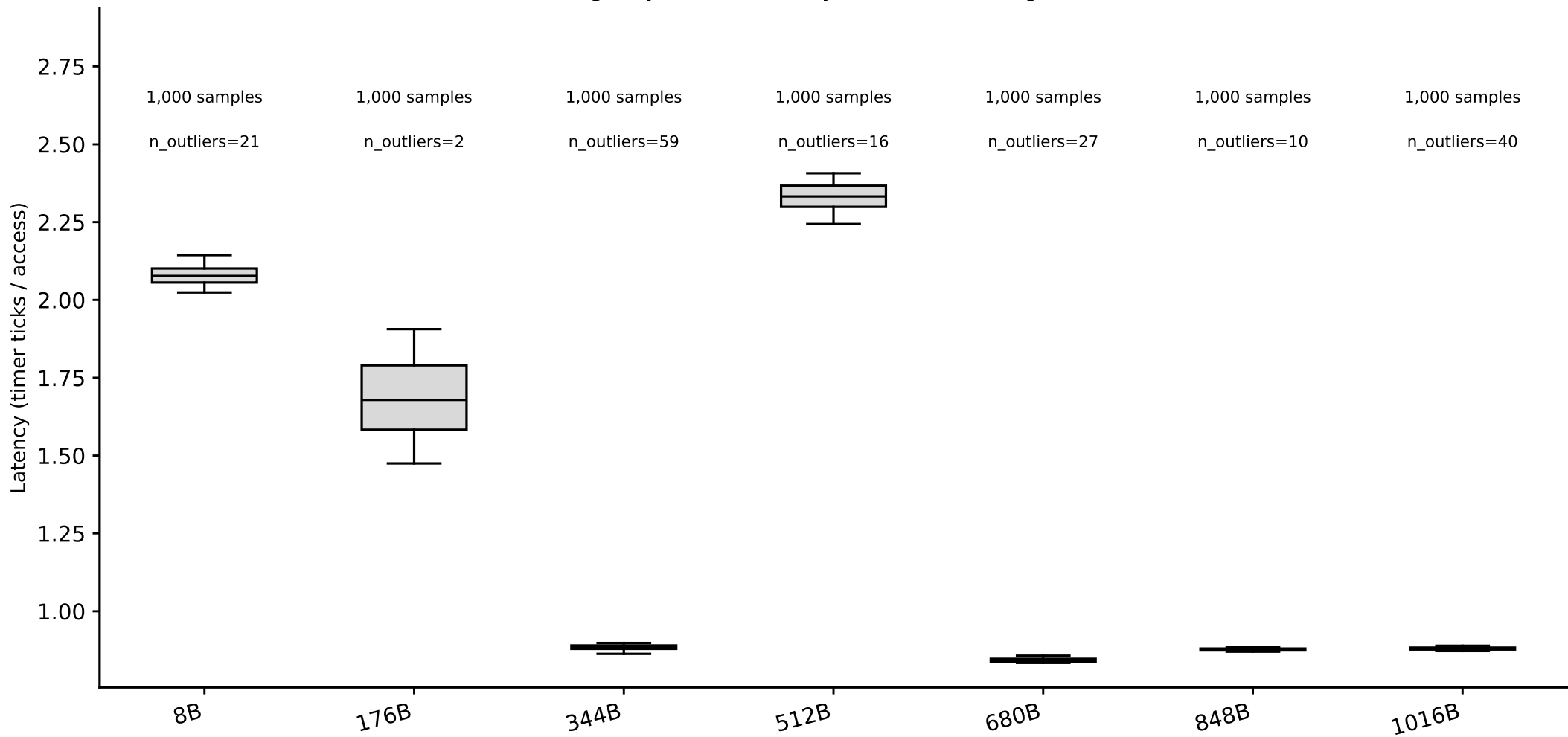
thunderbird: line-size box plots, random pattern (whiskers = p5/p95) (Phase I timing-only, level boundary=31457280B, single-curve method)
