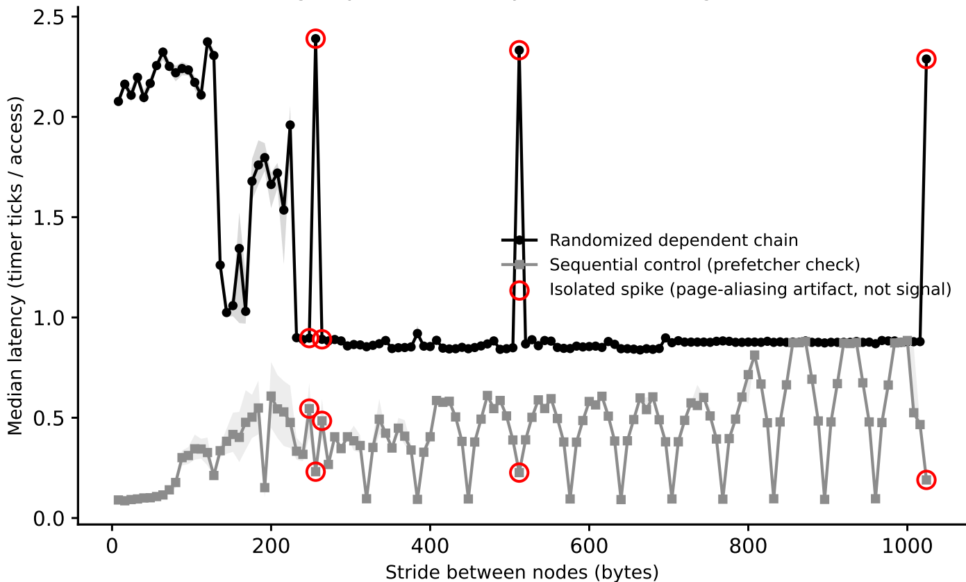
thunderbird: line-size sweep (dependent pointer chase), footprint=60 MiB (Phase I timing-only, level boundary=31457280B, single-curve method)
