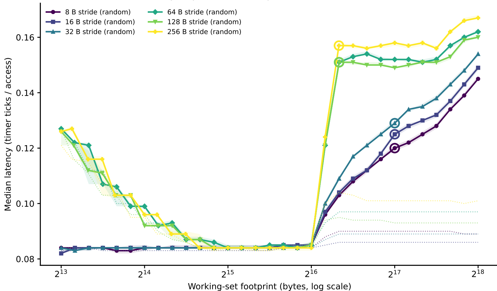
thunderbird: line-size family of curves (dependent pointer chase) (Phase I timing-only, level boundary=65536B window=[8192,262144])
