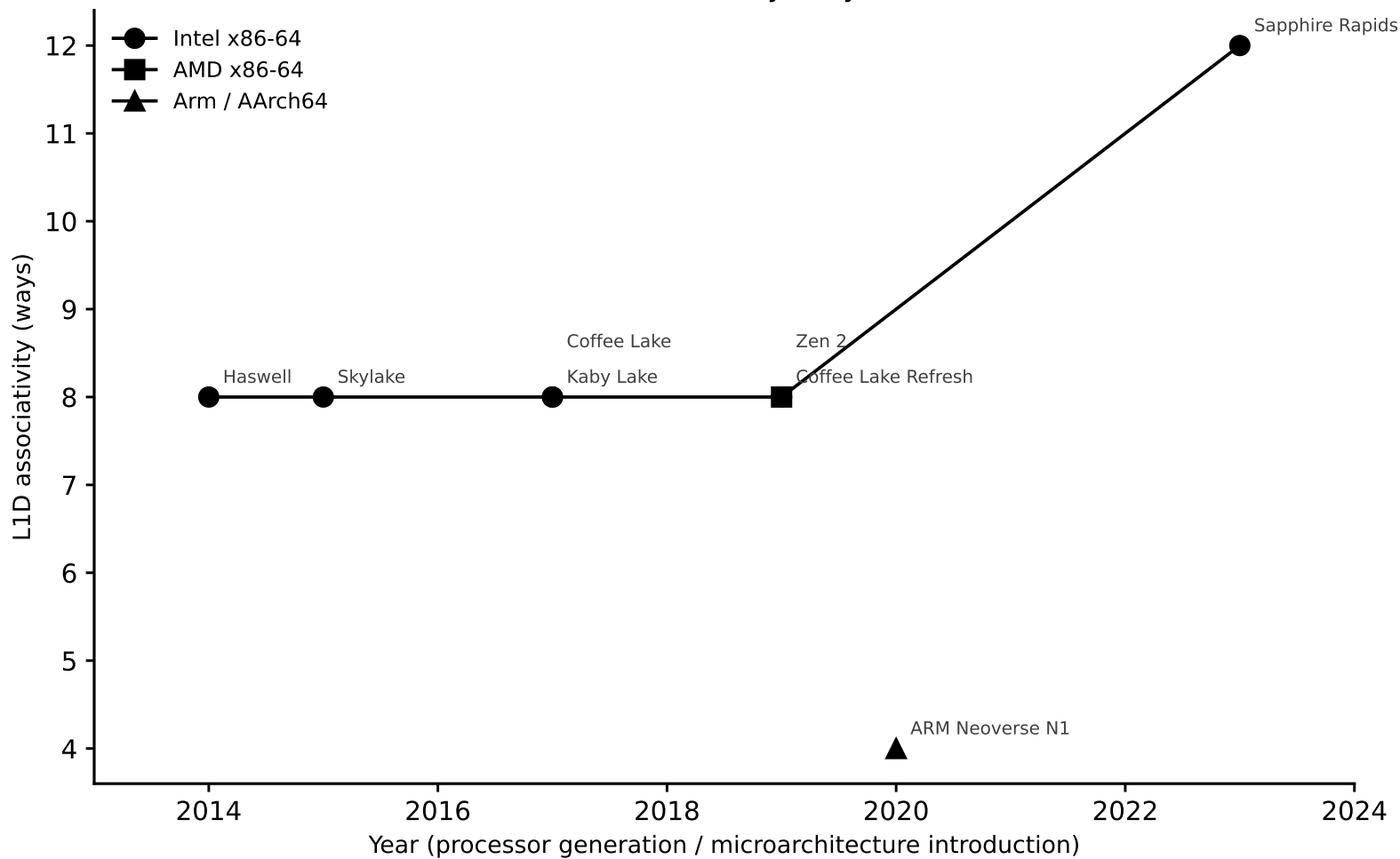
L1D associativity vs. year
