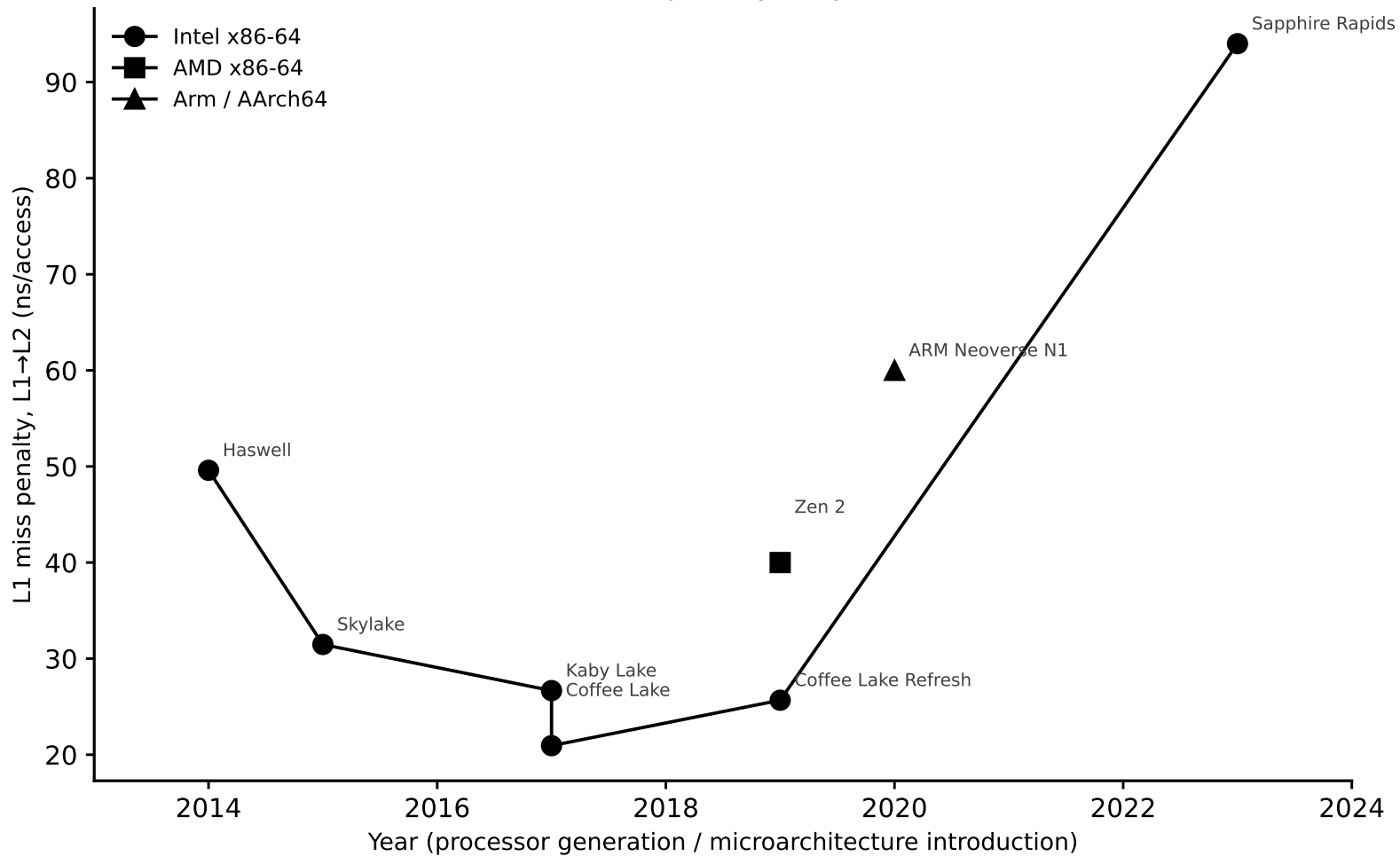
L1 miss penalty vs. year
