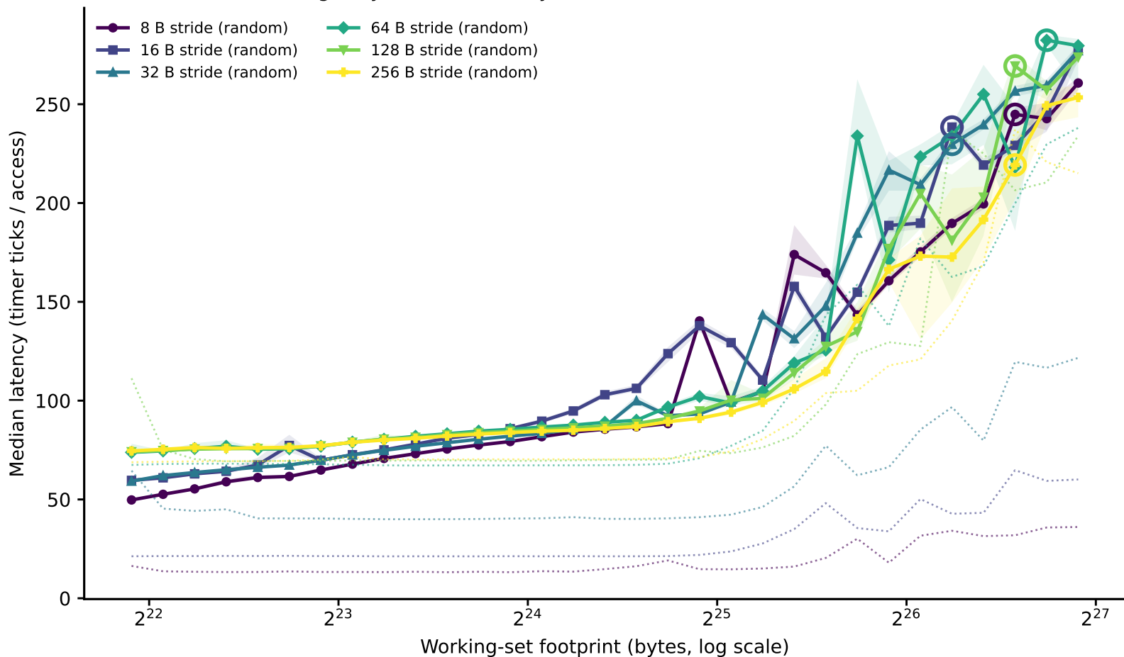
artemisia: line-size family of curves (dependent pointer chase) (Phase I timing-only, level boundary=31457280B window=[3932160,125829120])
