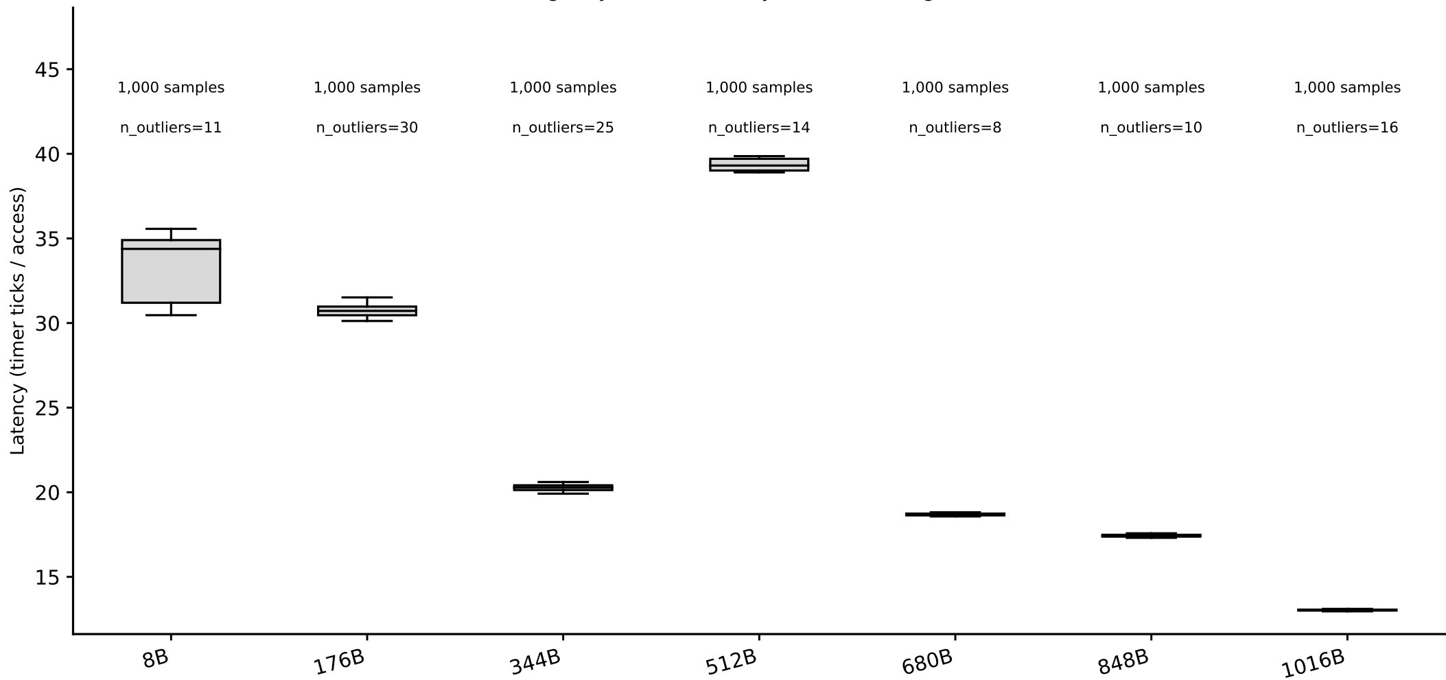
charnwood: line-size box plots, random pattern (whiskers = p5/p95) (Phase I timing-only, level boundary=262144B, single-curve method)
