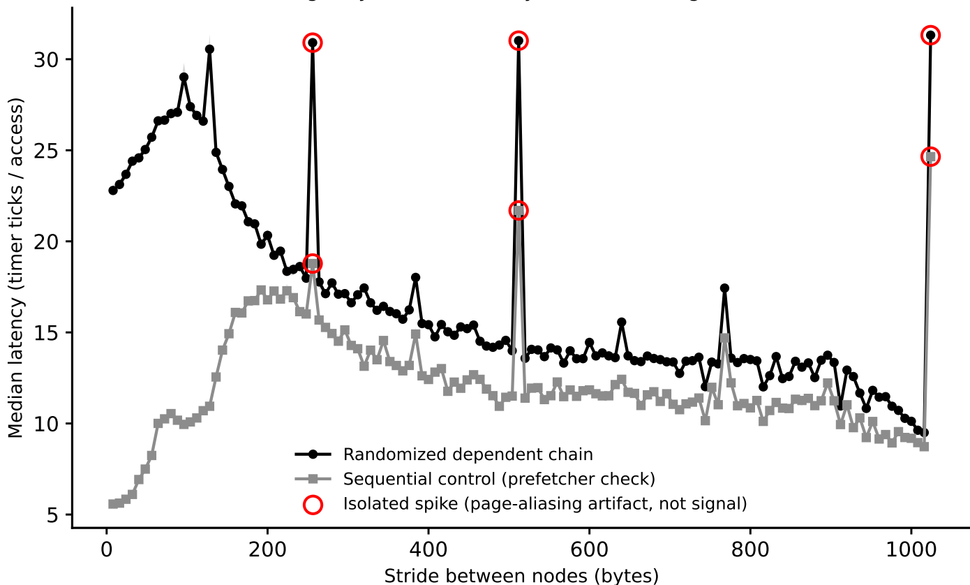
crux: line-size sweep (dependent pointer chase), footprint=512 KiB (Phase I timing-only, level boundary=262144B, single-curve method)
