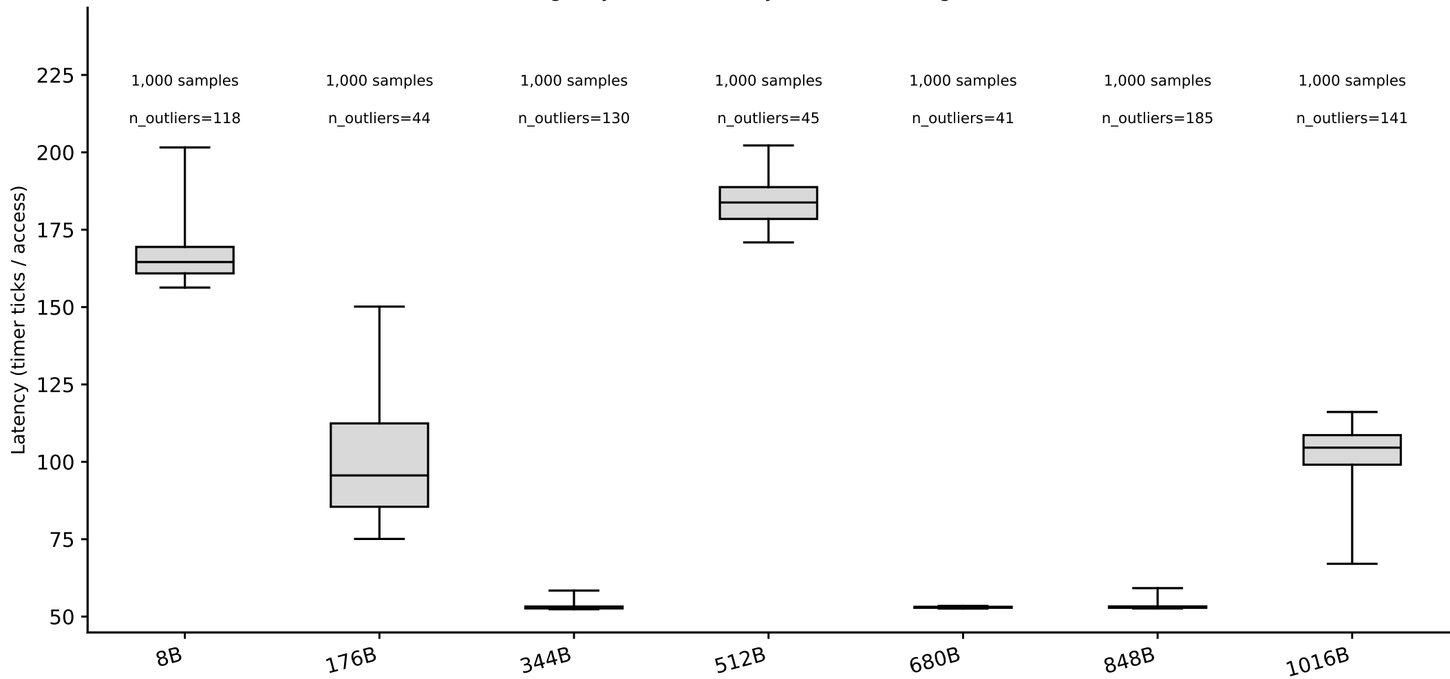
ookay: line-size box plots, random pattern (whiskers = p5/p95) (Phase I timing-only, level boundary=8388608B, single-curve method)
