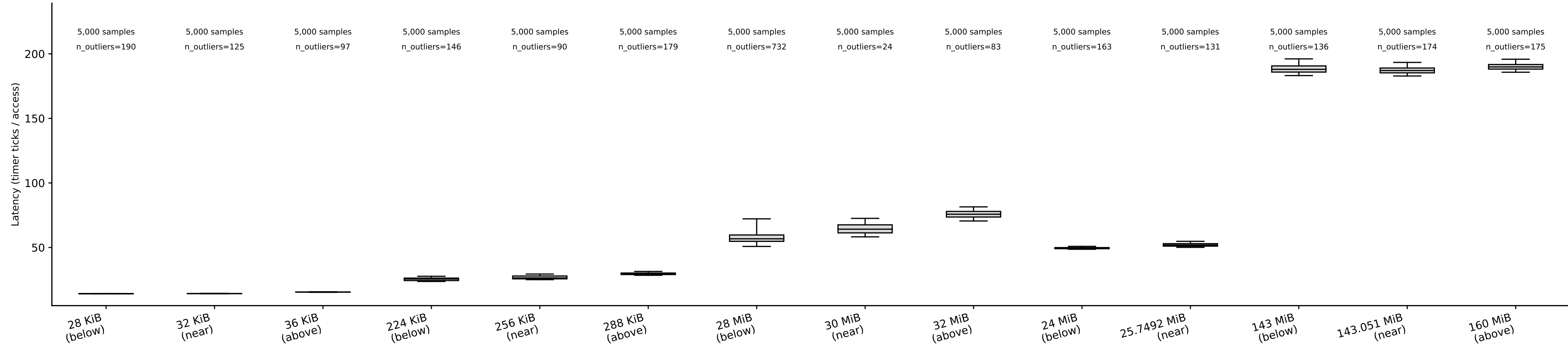
sunbird: capacity box plots, random pattern (whiskers = p5/p95) (Phase I timing-only, targeted discrete-size validation, core 6) tested boundaries: 32 KiB, 256 KiB, 30 MiB, 25.7492 MiB, 143.051 MiB
