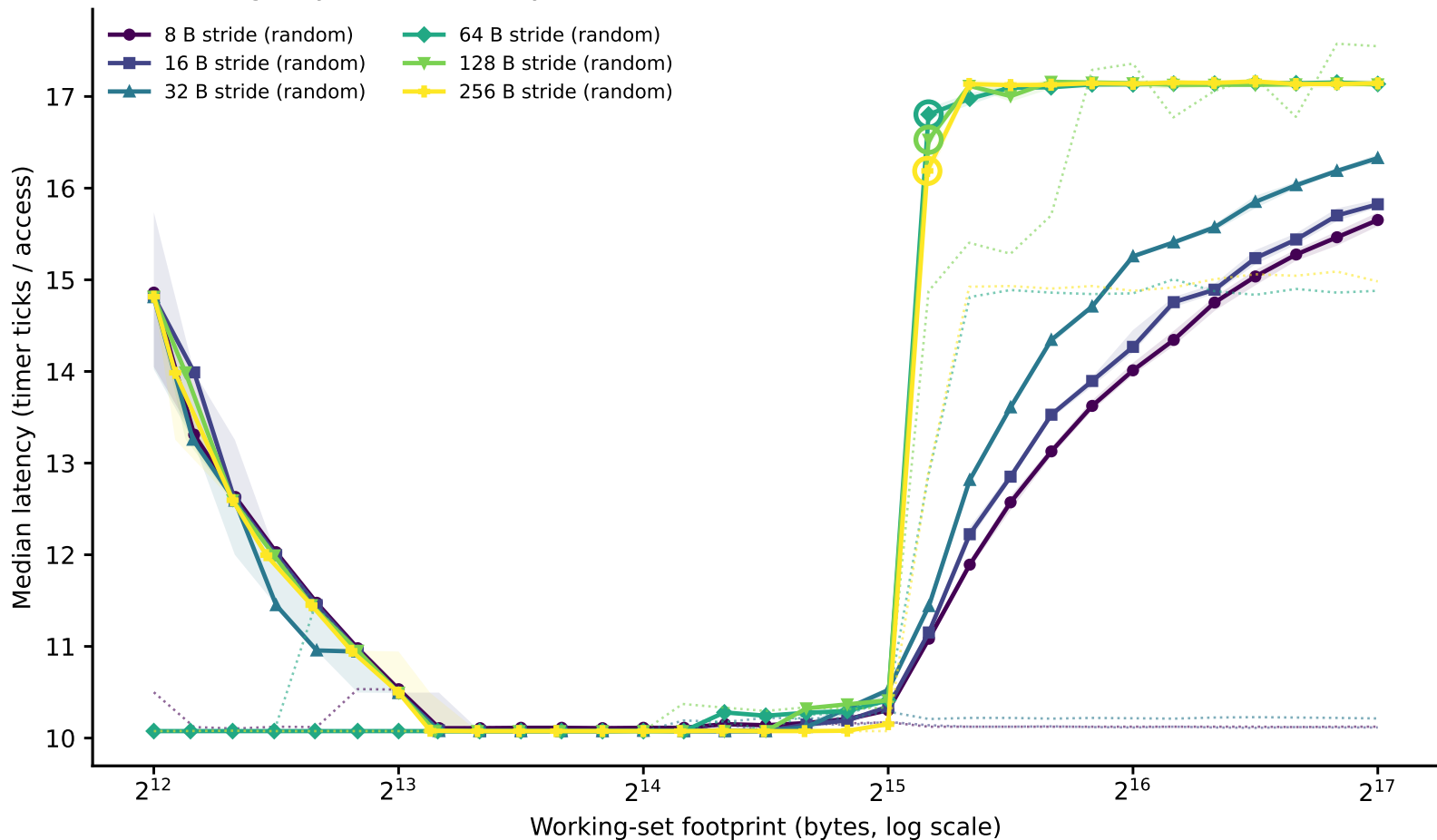
sunbird: line-size family of curves (dependent pointer chase) (Phase I timing-only, level boundary=32768B window=[4096,131072], fresh re-run 20260912T222501Z)
