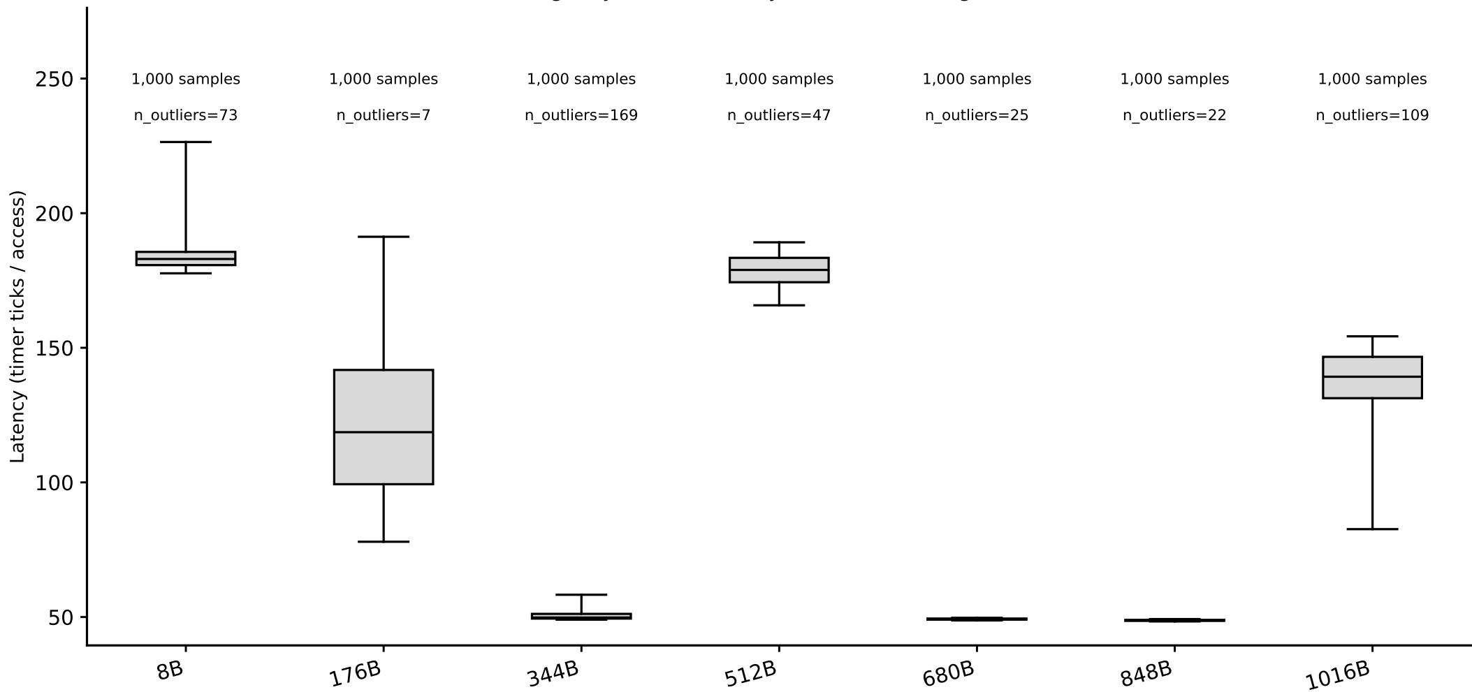
upgrade: line-size box plots, random pattern (whiskers = p5/p95) (Phase I timing-only, level boundary=12582912B, single-curve method)
