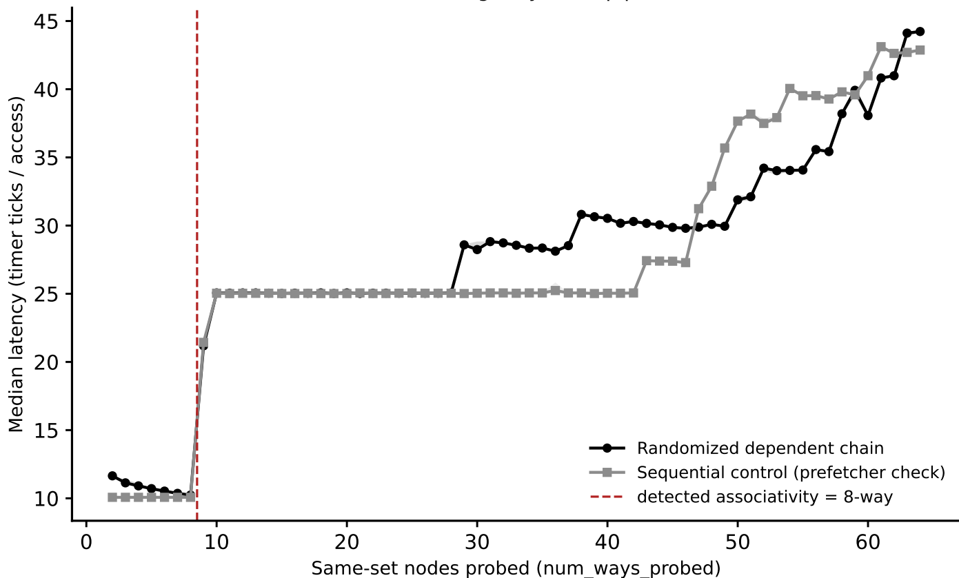
sunbird: associativity sweep, L1 (stride=32 KiB) (Phase I timing-only, auto pipeline)
