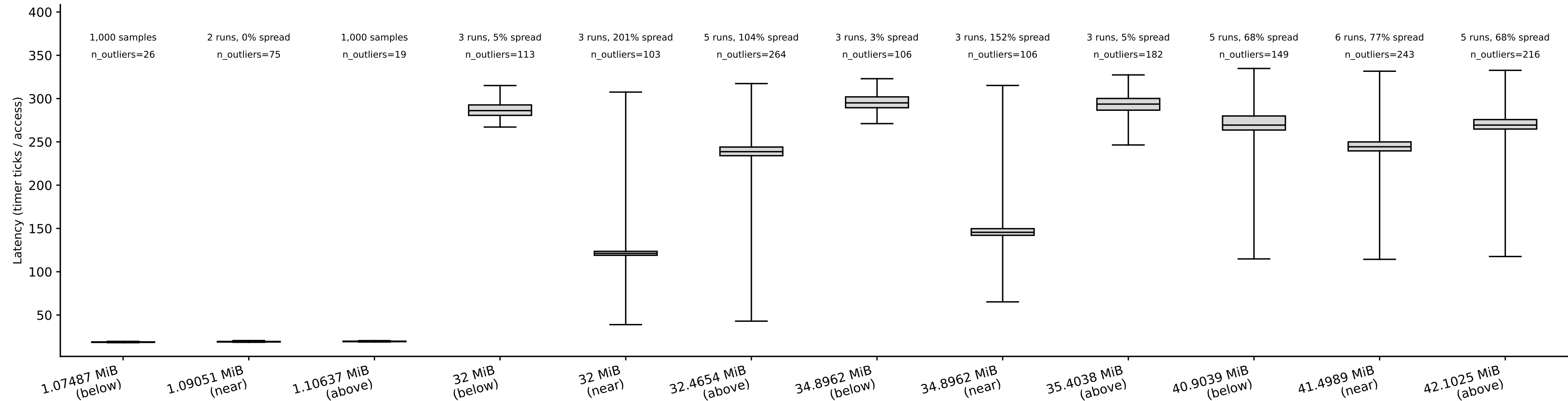
hazel_turin: capacity box plots, random pattern (whiskers = p5/p95) (Phase I timing-only, auto pipeline) tested boundaries: 1.09051 MiB, 32 MiB, 34.8962 MiB, 41.4989 MiB
