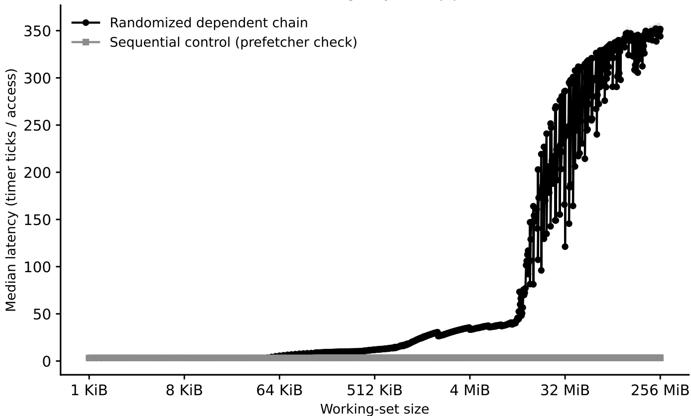
hazel_turin: capacity sweep (dependent pointer chase) (Phase I timing-only, auto pipeline)
