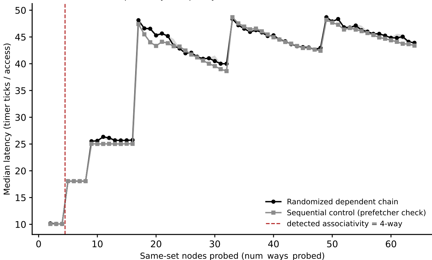
sunbird: associativity sweep, L2_candidate_128KiB (stride=128 KiB) (exploratory -- capacity NOT confirmed, see README)
