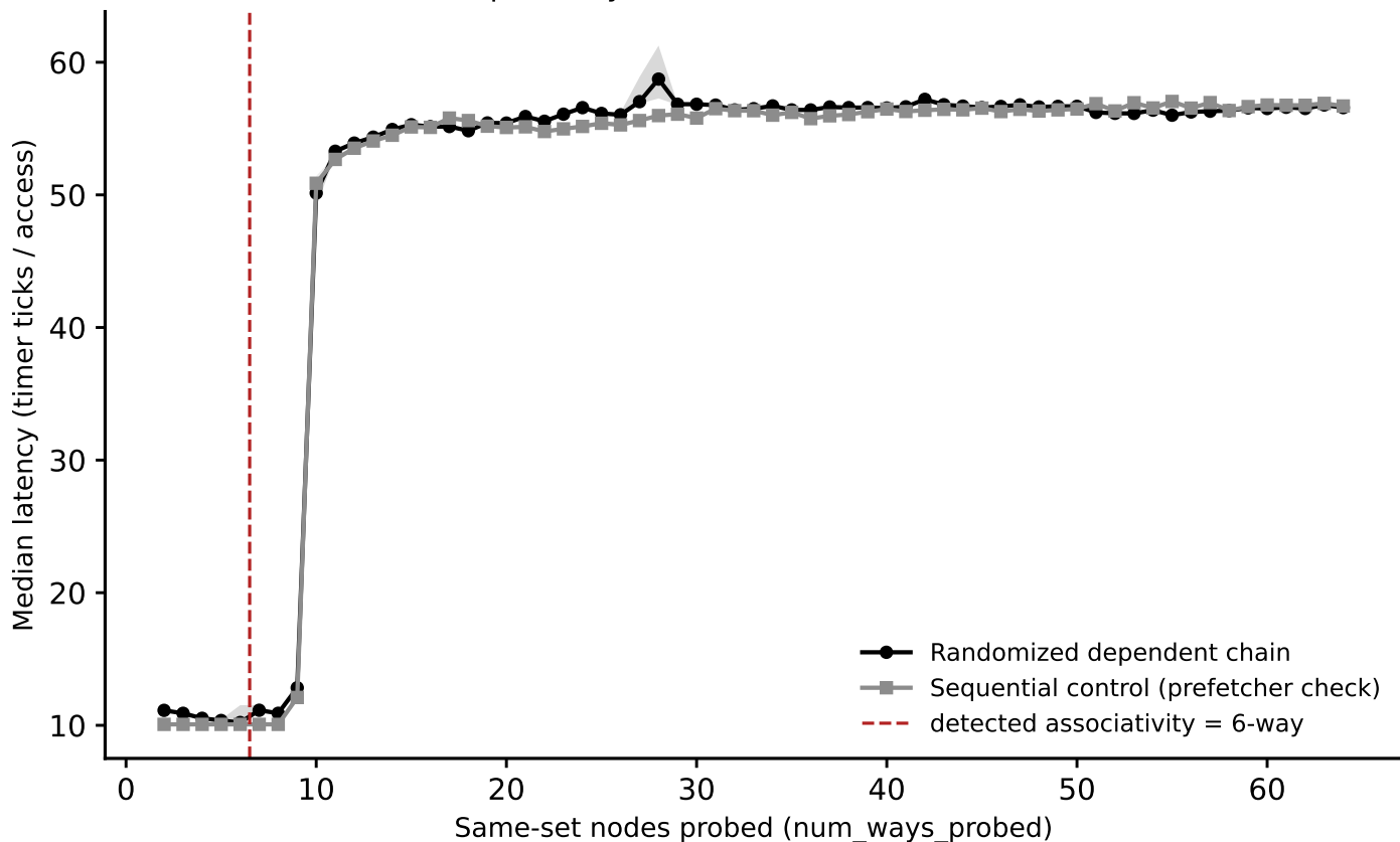
sunbird: associativity sweep, LLC_candidate_16MiB (stride=16 MiB) (exploratory -- inconclusive, see README)
