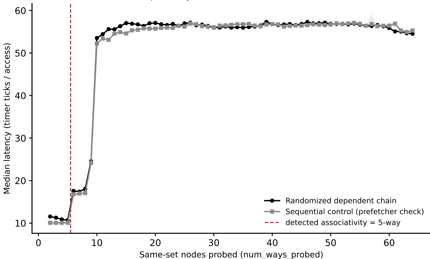
sunbird: associativity sweep, LLC_candidate_32MiB (stride=32 MiB) (exploratory -- inconclusive, see README)
