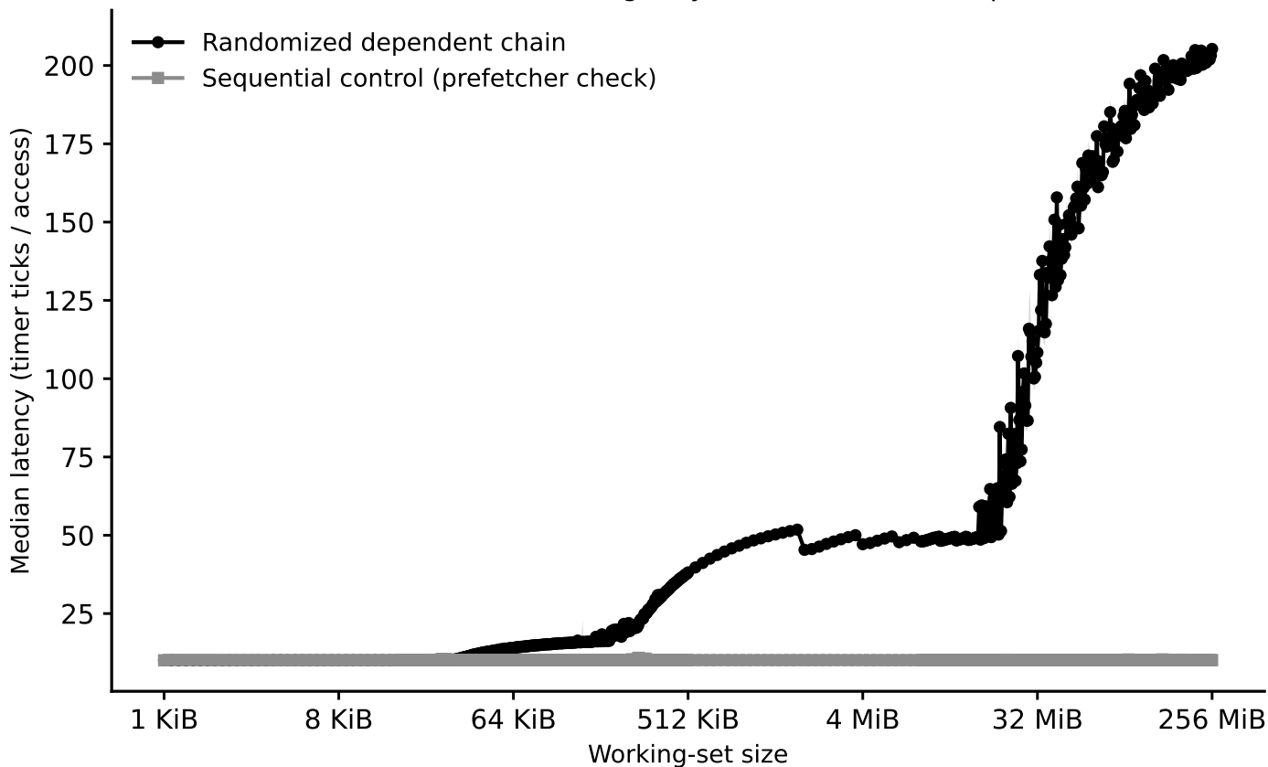
sunbird: capacity sweep (dependent pointer chase) (Xeon E5-2680 v3, Phase I timing-only, 1KiB-256MiB, 3-4 reps 16-256MiB)
