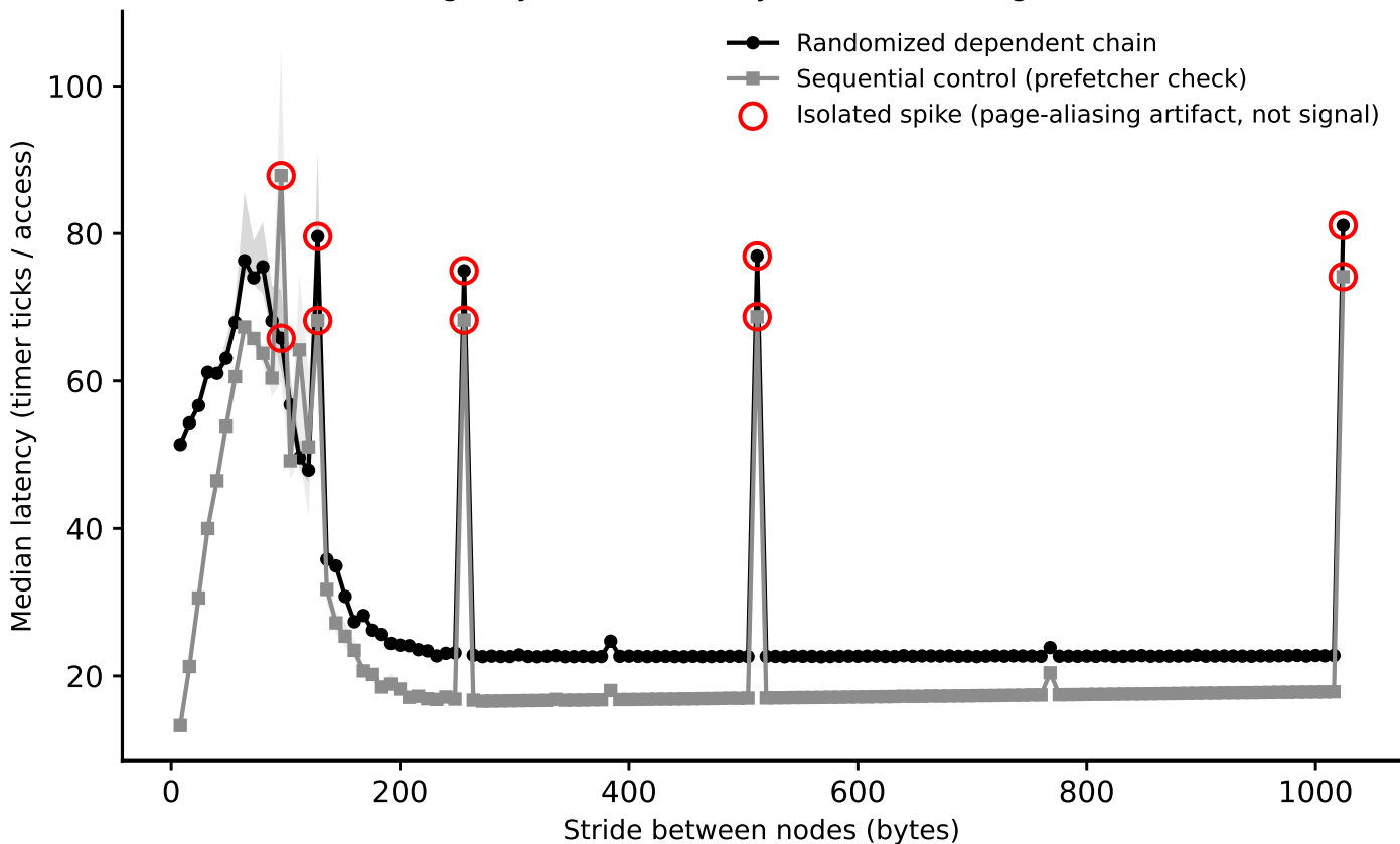
artemisia: line-size sweep (dependent pointer chase), footprint=4 MiB (Phase I timing-only, level boundary=2097152B, single-curve method)
