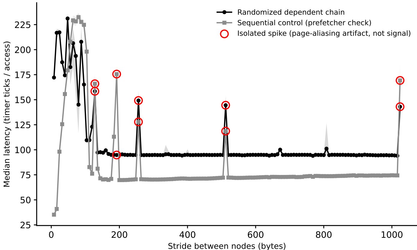
artemisia: line-size sweep (dependent pointer chase), footprint=60 MiB (Phase I timing-only, level boundary=31457280B, single-curve method)
