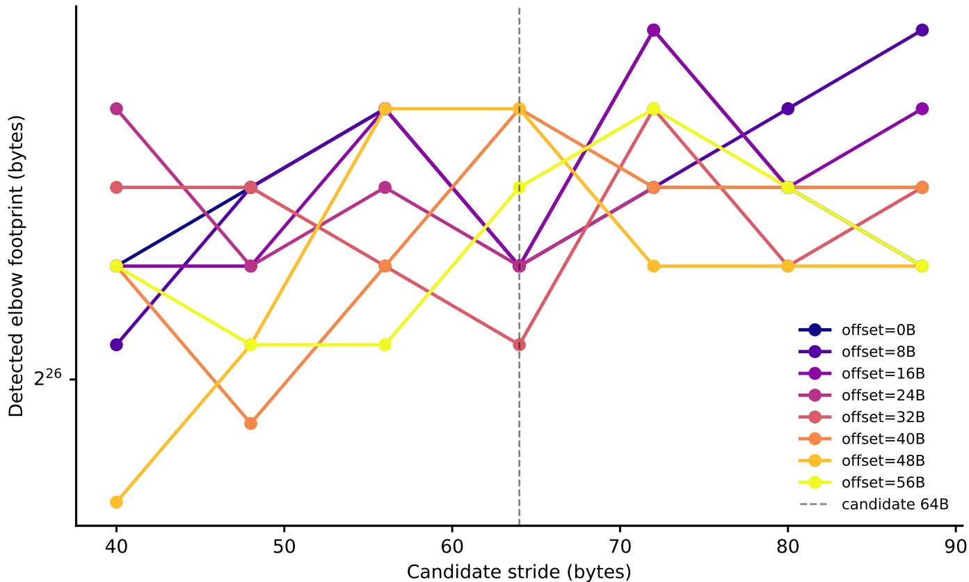
artemisia: line-size elbow vs. stride, by node-0 offset (Phase I timing-only, level boundary=31457280B, step-4 alignment refinement)
