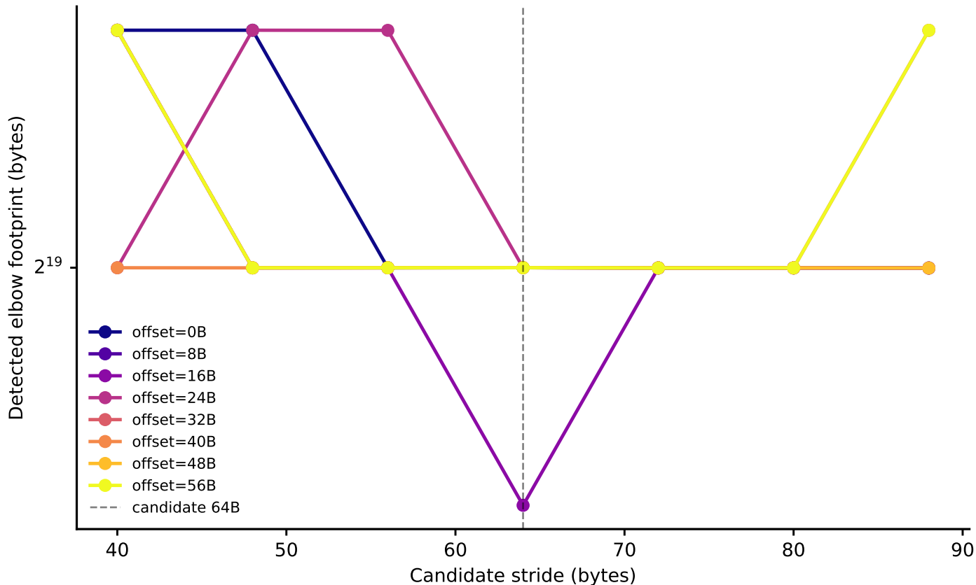
crux: line-size elbow vs. stride, by node-0 offset (Phase I timing-only, level boundary=262144B, step-4 alignment refinement)
