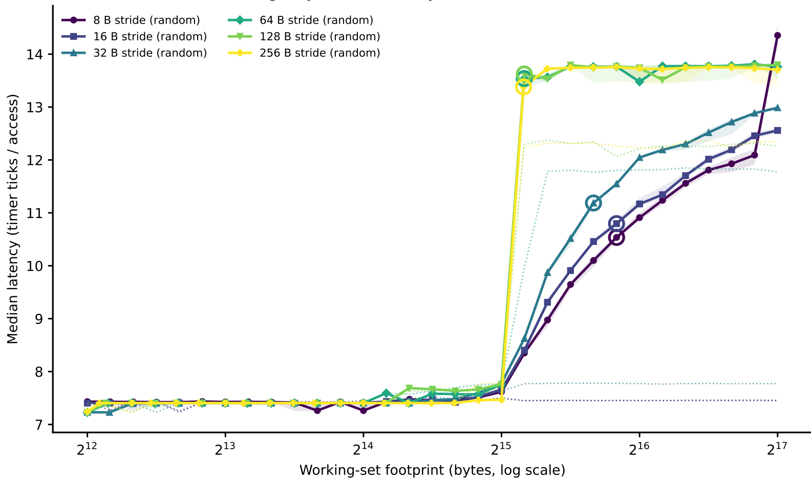
ookay: line-size family of curves (dependent pointer chase) (Phase I timing-only, level boundary=32768B window=[4096,131072])
