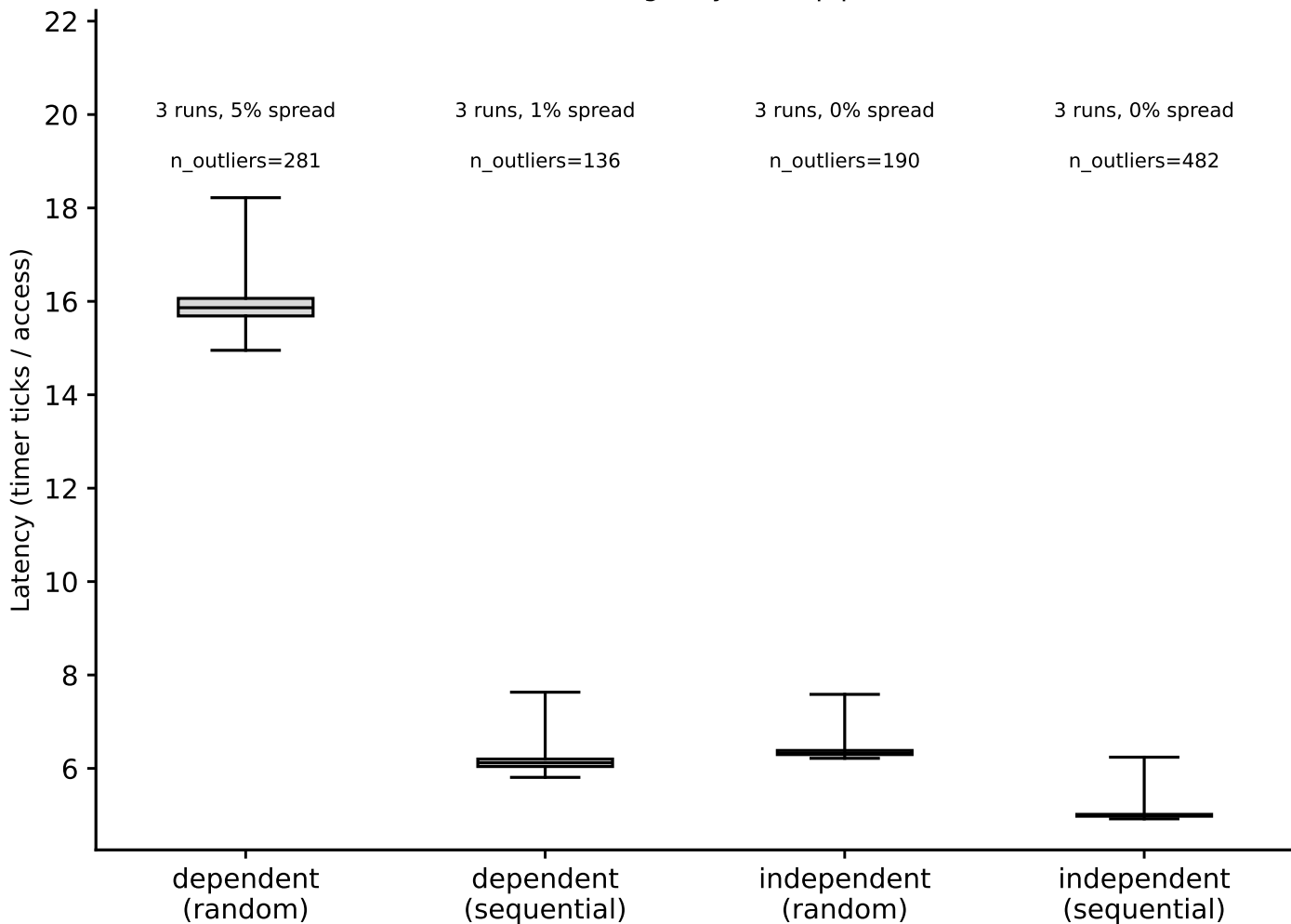
skylark: hit-latency box plots, L2 (footprint=512 KiB) (Phase I timing-only, auto pipeline)
