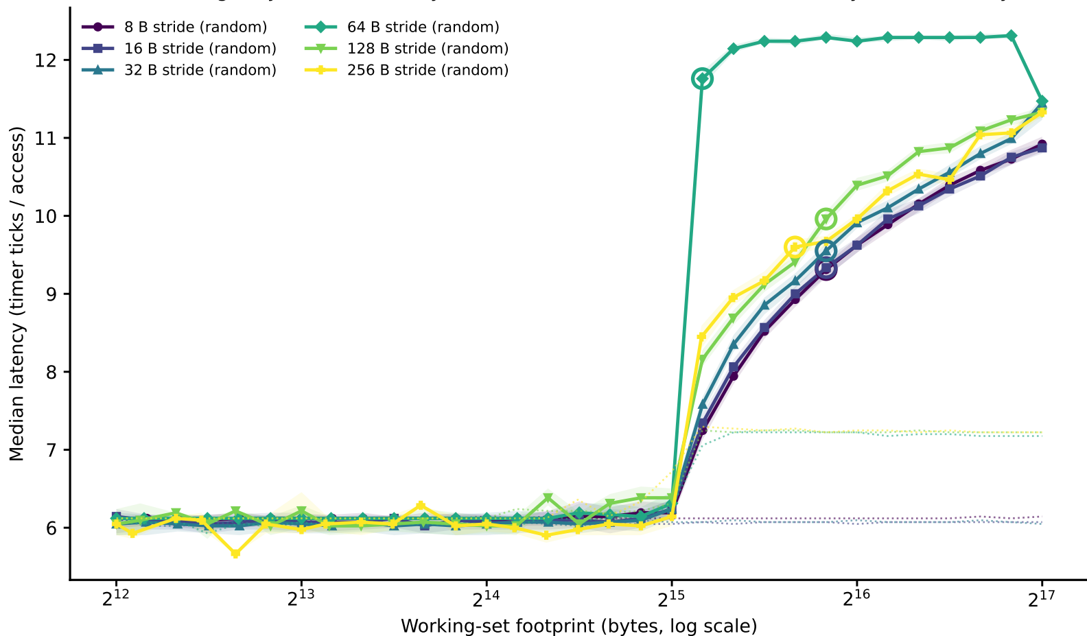
skylark: line-size family of curves (dependent pointer chase) (Phase I timing-only, level boundary=32768B window=[4096,131072], family-of-curves-only rerun)
