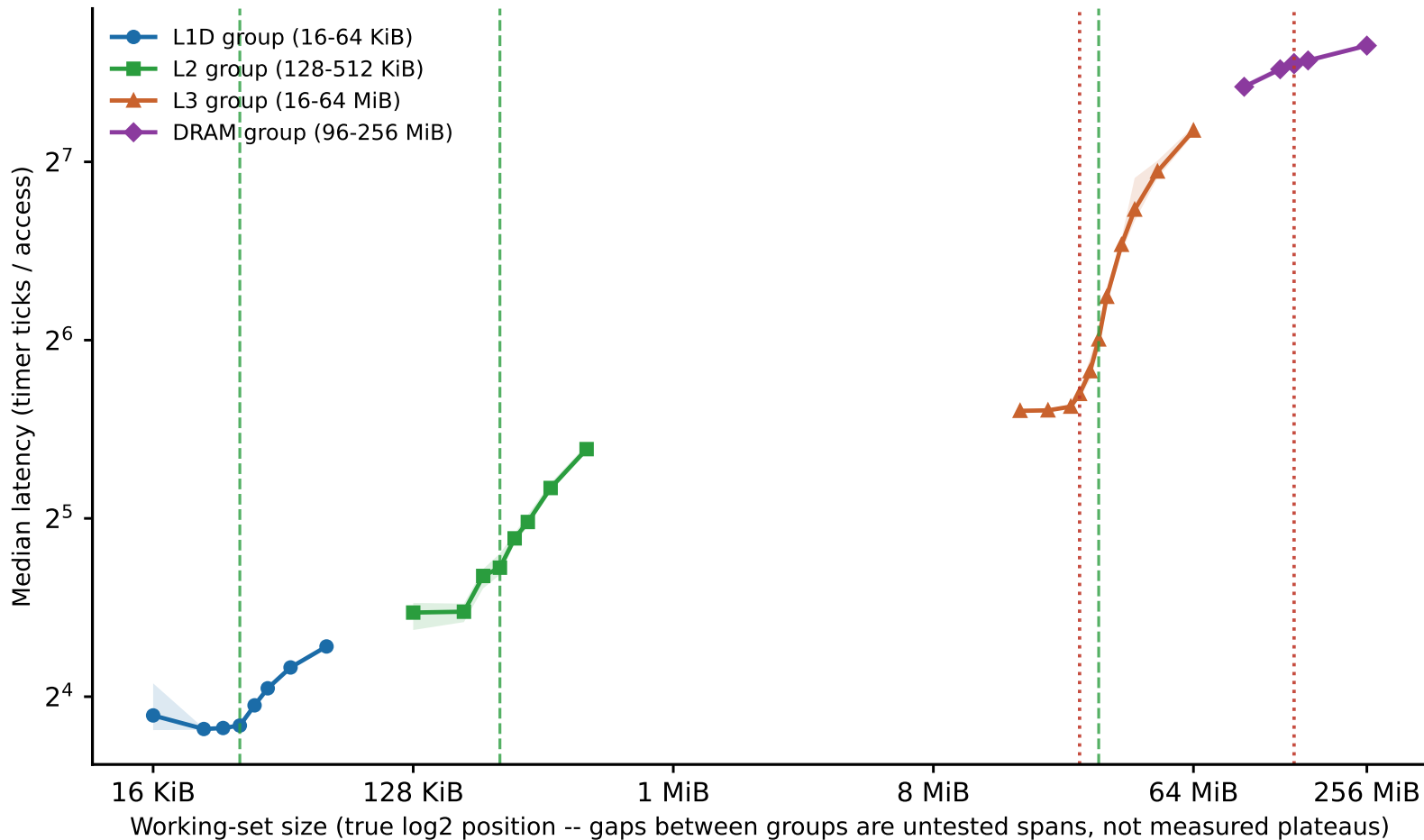
sunbird: capacity_validate, expected (green --) vs. flagged (red :) boundaries (Phase I timing-only, targeted discrete-size validation, core 6)
