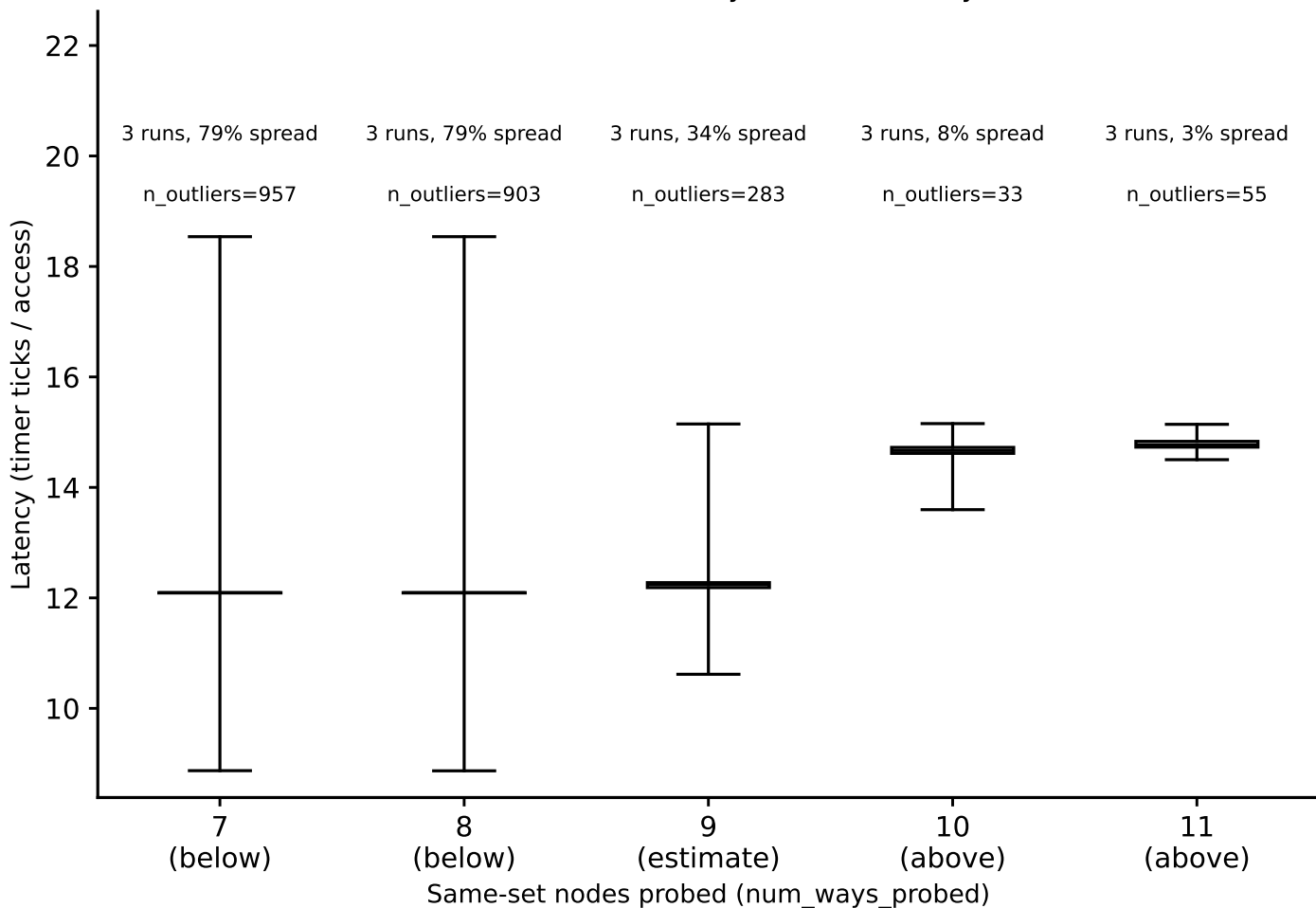
hazel_broadwell: associativity box plots, L3_LLC, random pattern (whiskers = p5/p95) (Phase I timing-only, auto pipeline) detected associativity estimate: 9-way
