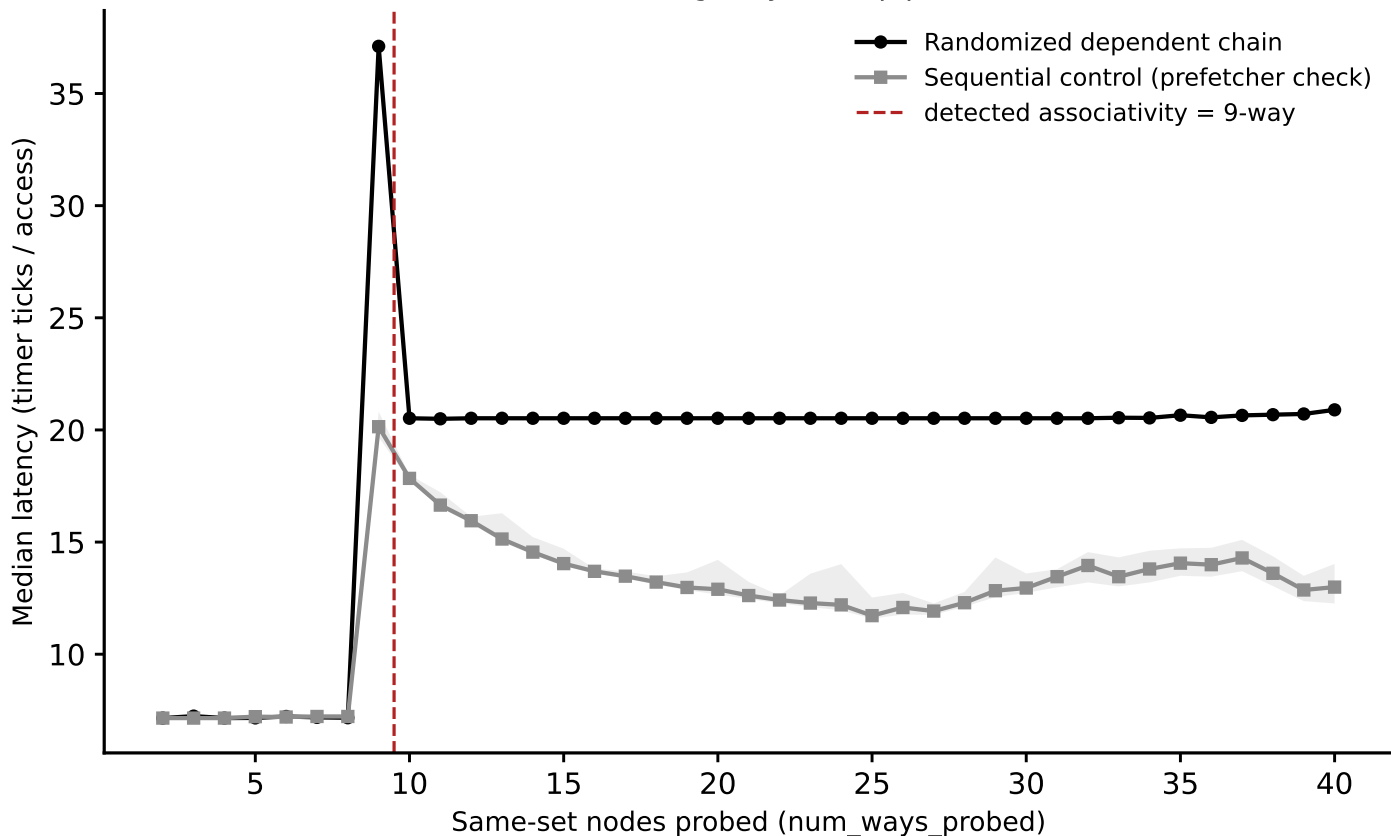
hazel_genoa: associativity sweep, L1 (stride=32 KiB) (Phase I timing-only, auto pipeline)
