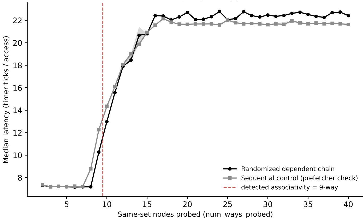
hazel_genoa: associativity sweep, L3_LLC (stride=32 MiB) (Phase I timing-only, auto pipeline)
